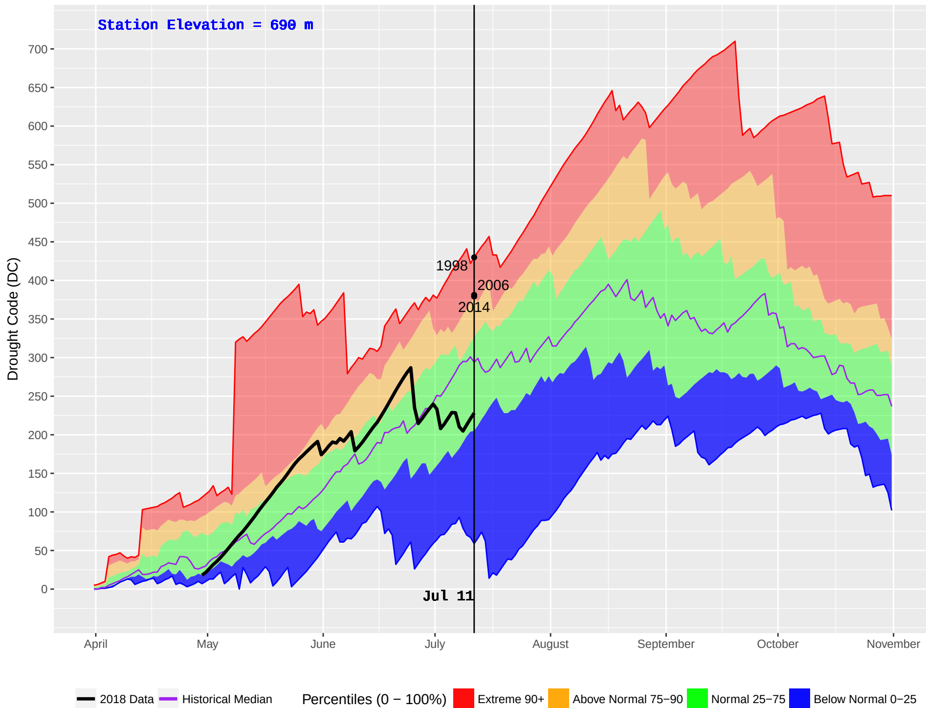
MACKENZIE FS (155) : Historical (1994–2016) and Current (2018) Noon Drought Code (DC)
