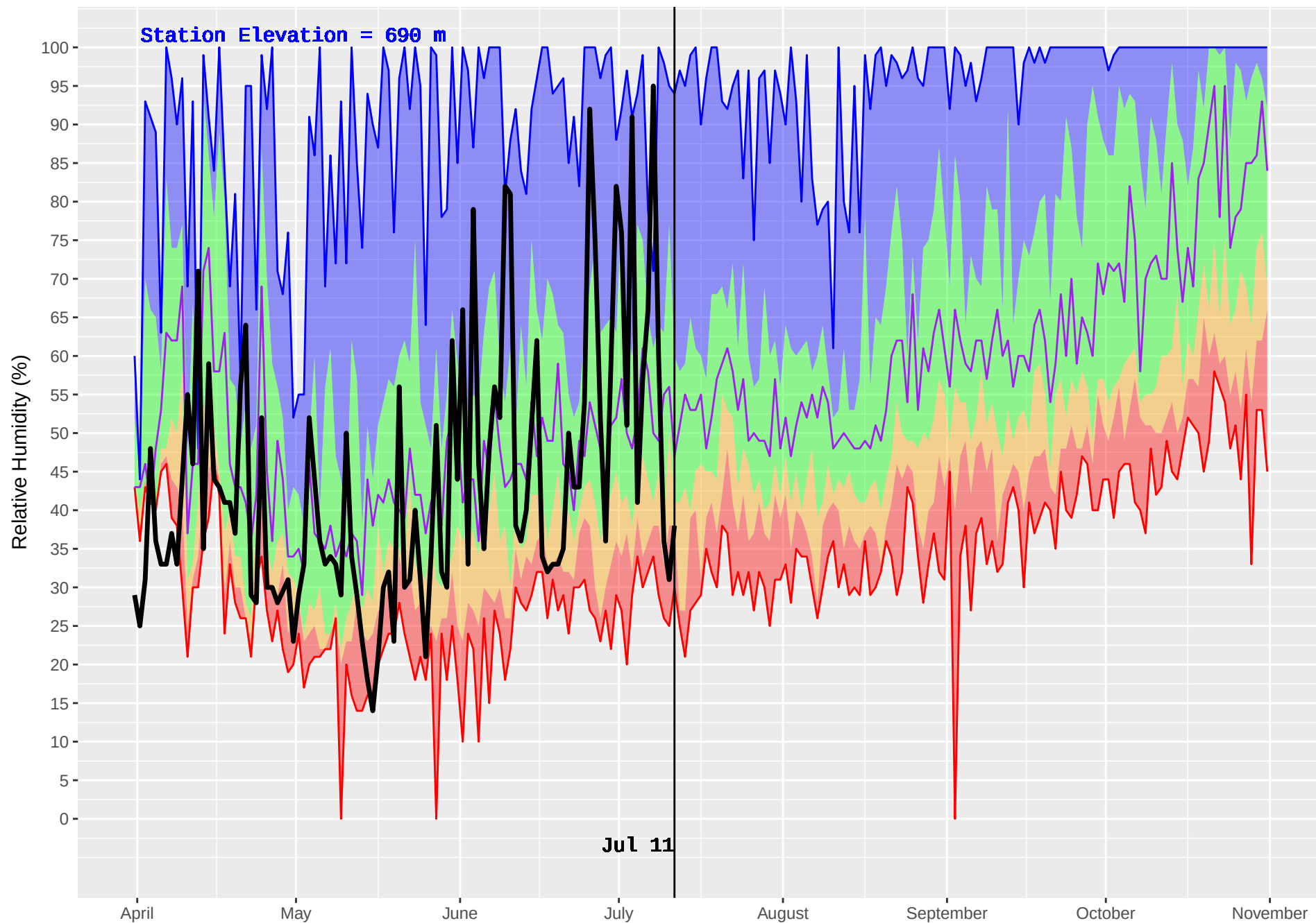
MACKENZIE FS (155) : Historical (1994–2016) and Current (2018) Noon Relative Humidity
