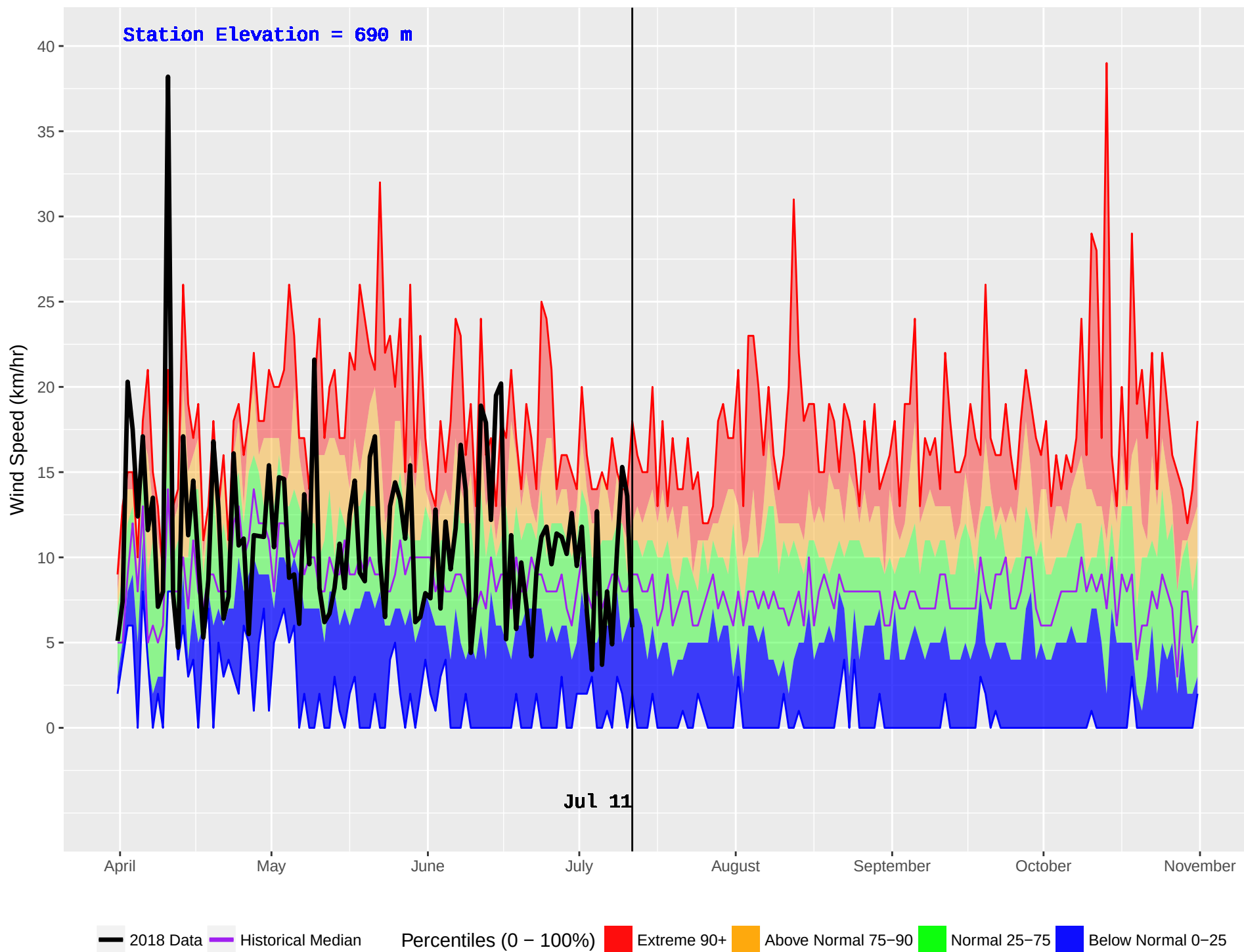
MACKENZIE FS (155) : Historical (1994–2016) and Current (2018) Noon Wind Speed
